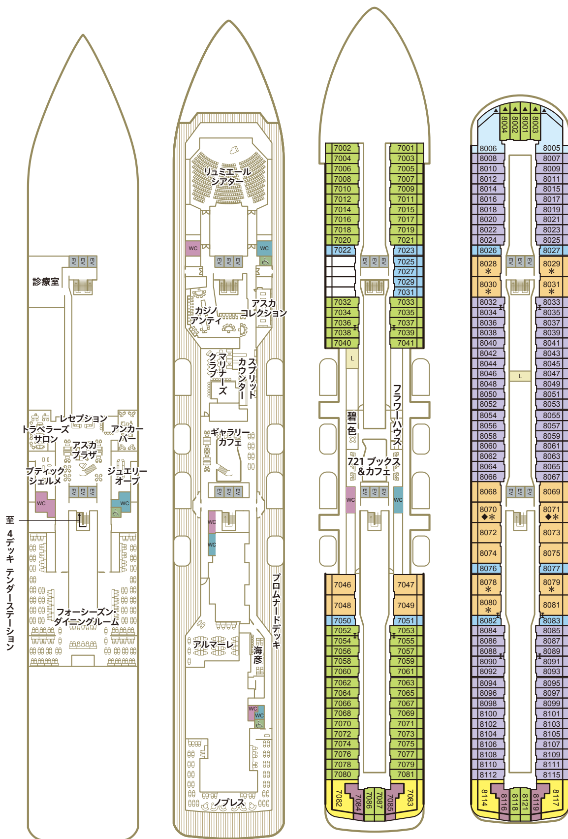
DECK 5
